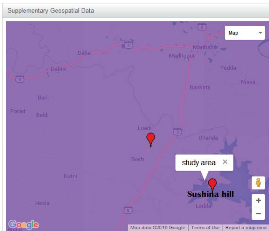
Figure 1: Location map of the Sushina hill.
